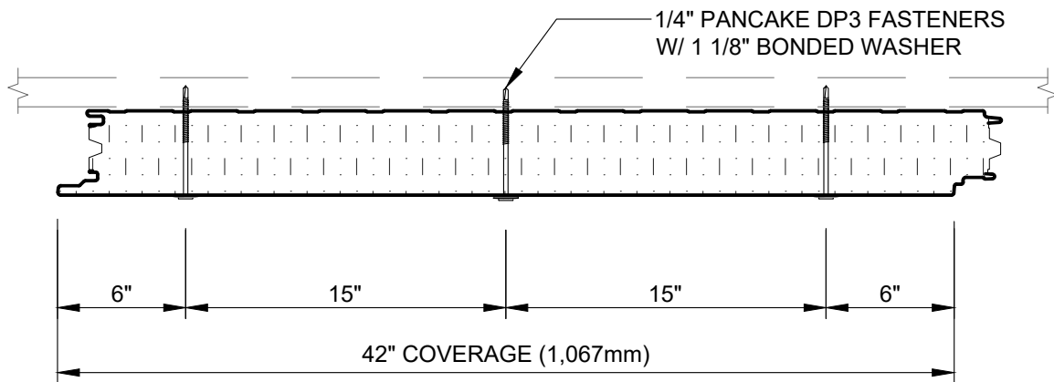
THROUGH FASTENING REQUIREMENTS (3 - THROUGH FASTENER PATTERN EXAMPLE)
