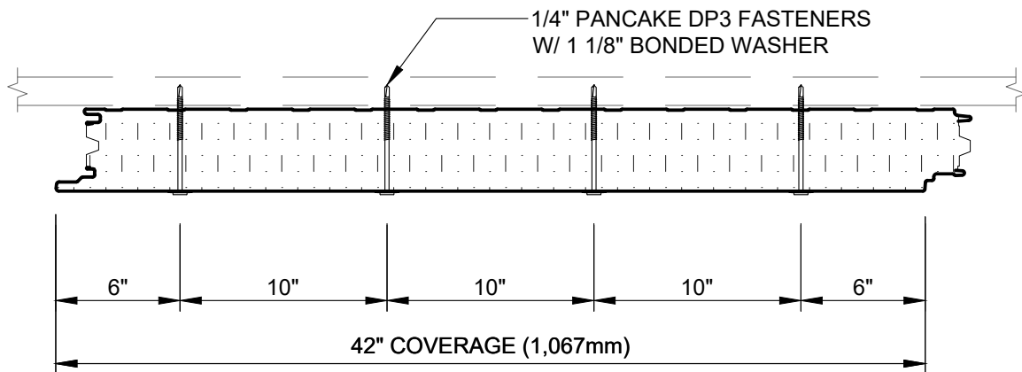
THROUGH FASTENING REQUIREMENTS (4 - THROUGH FASTENER PATTERN EXAMPLE)
