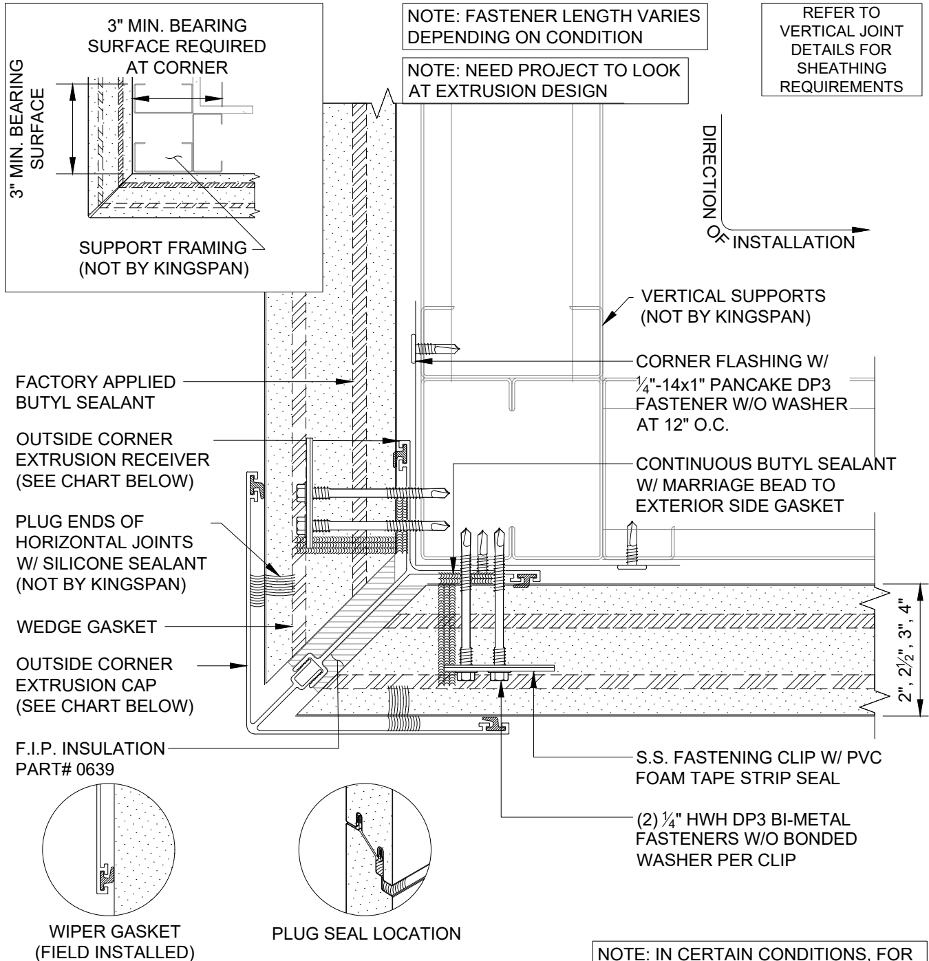
CORNER EXTRUSION PART NUMBERS
