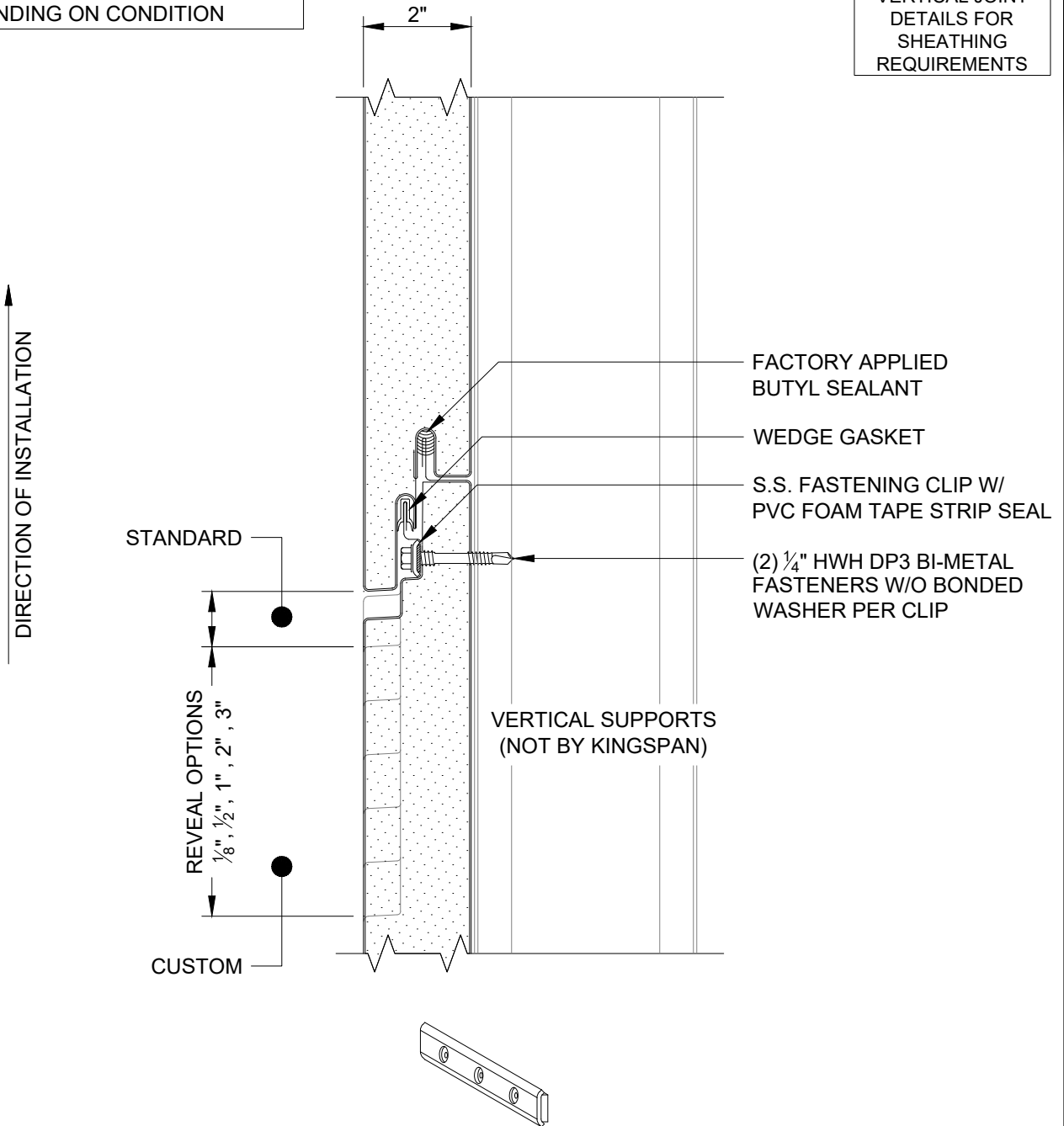
FASTENING CLIP
