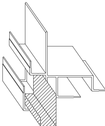
SPLICE PLATE FOR OUTSIDE CORNER EXTRUSION
