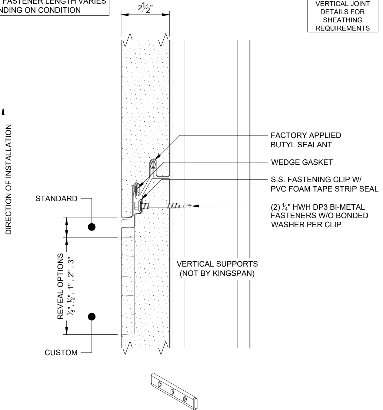
FASTENING CLIP
