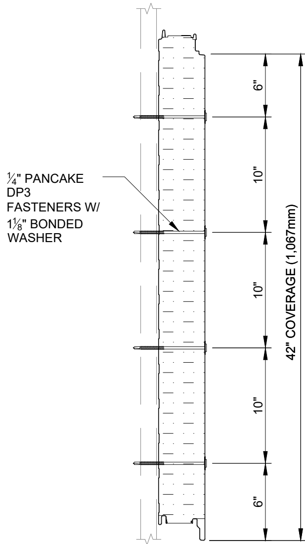
THROUGH FASTENING REQUIREMENTS (4 - THROUGH FASTENER PATTERN EXAMPLE)
