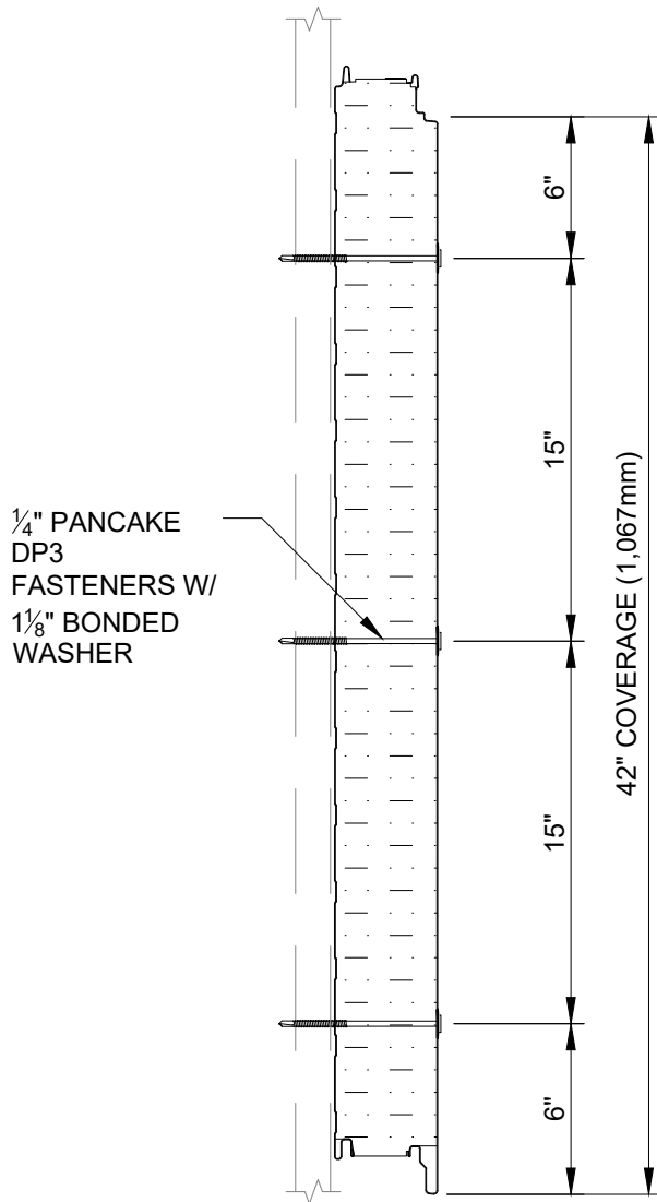
THROUGH FASTENING REQUIREMENTS (3 - THROUGH FASTENER PATTERN EXAMPLE)
