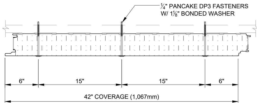
THROUGH FASTENING REQUIREMENTS (3 - THROUGH FASTENER PATTERN EXAMPLE)
