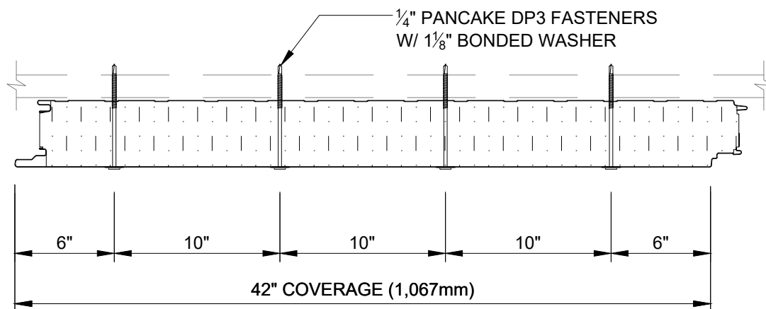
THROUGH FASTENING REQUIREMENTS (4 - THROUGH FASTENER PATTERN EXAMPLE)
